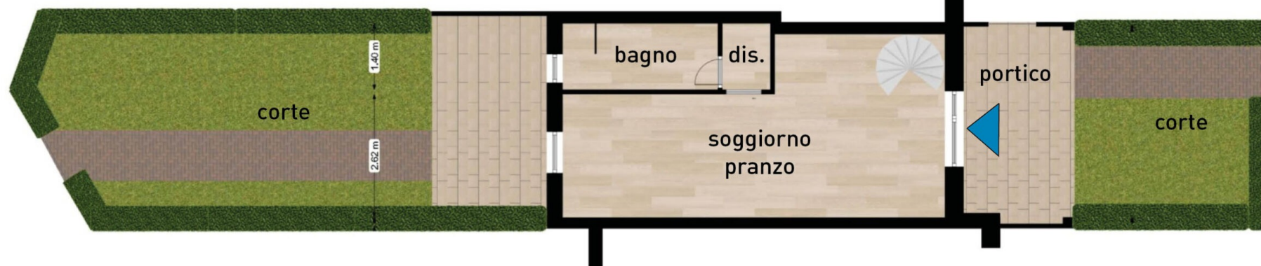
piano terra
